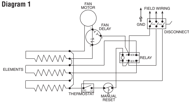
WIRING DIAGRAM FOR THREE PHASE WALL HEATERS
