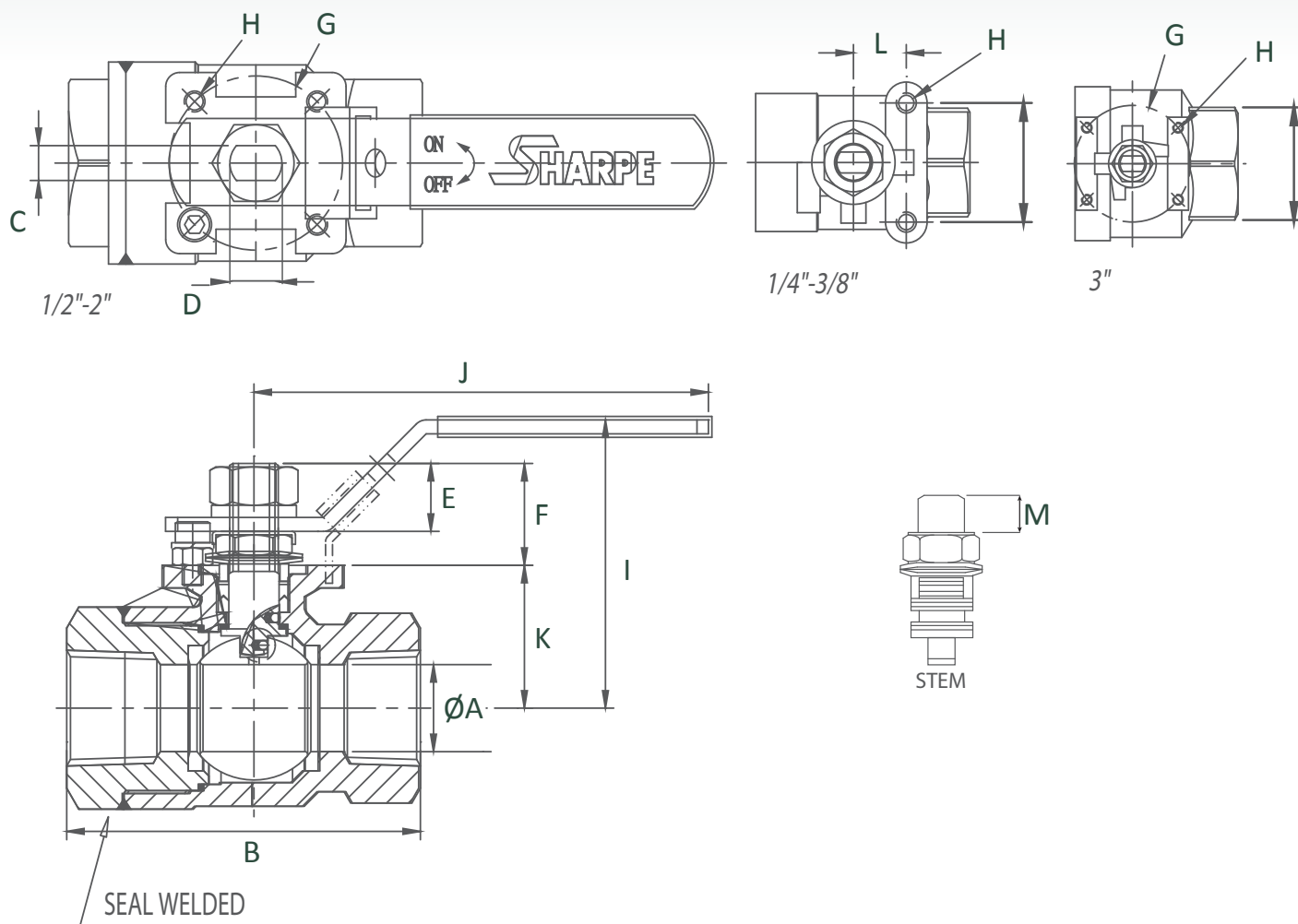
Dimensions (Inches)
