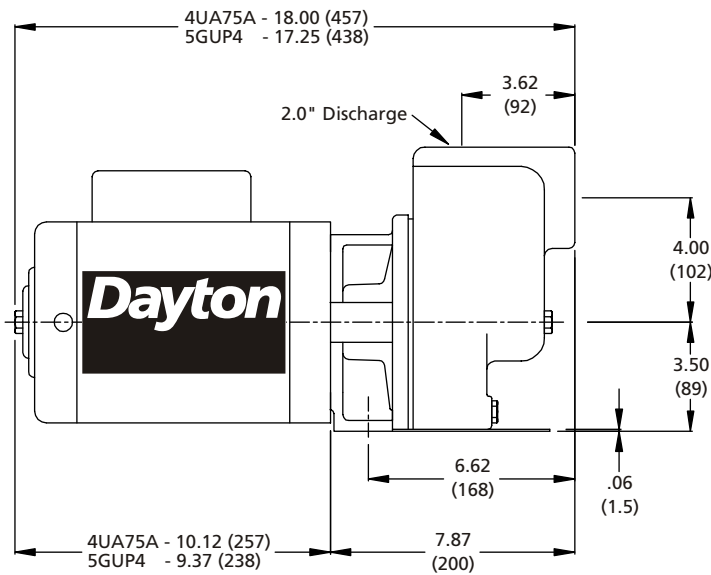
Figure 2 - Dimensions (mm)
