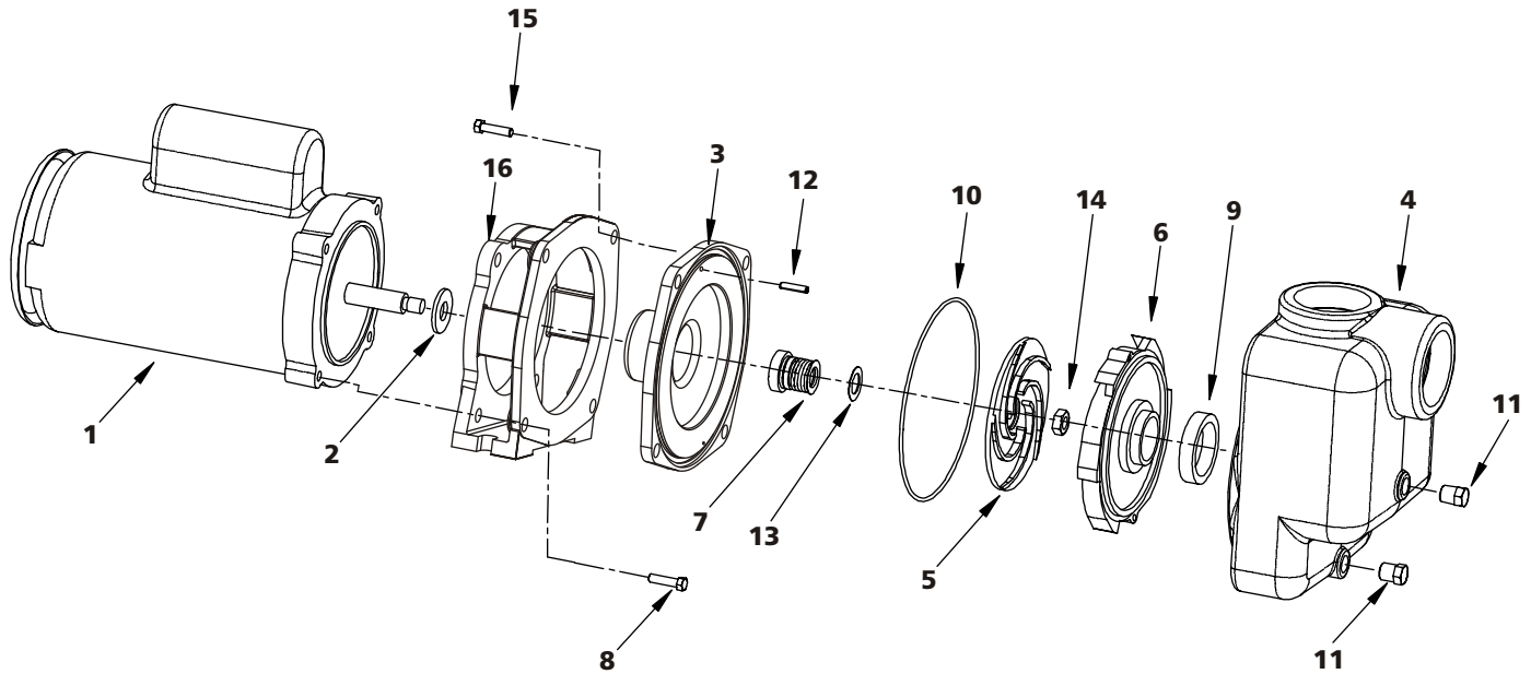
Figure 7 – Repair Parts Illustration
