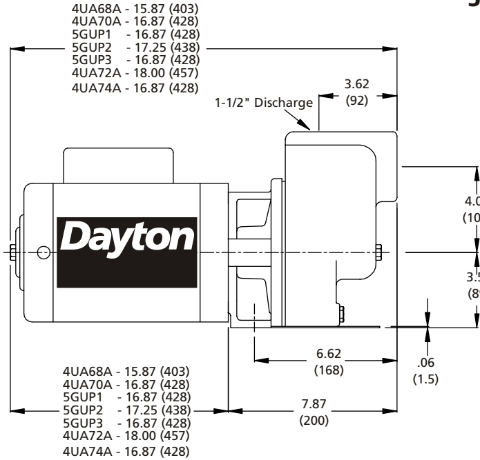
Figure 2 - Dimensions (mm)
