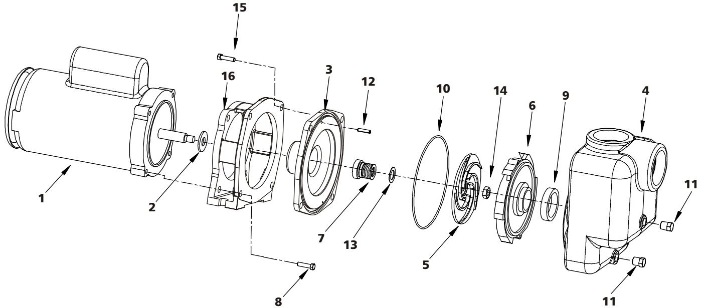
Figure 7 – Repair Parts Illustration
