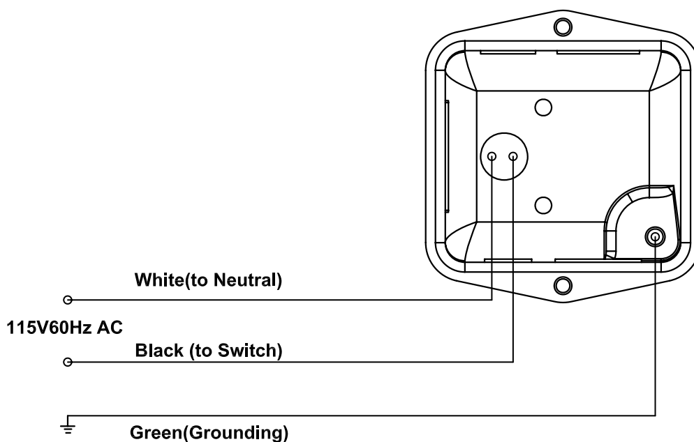
Figure 2 - Wiring Diagram. 115 volts connection.
